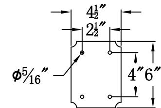
Front View of Mounting Plate
