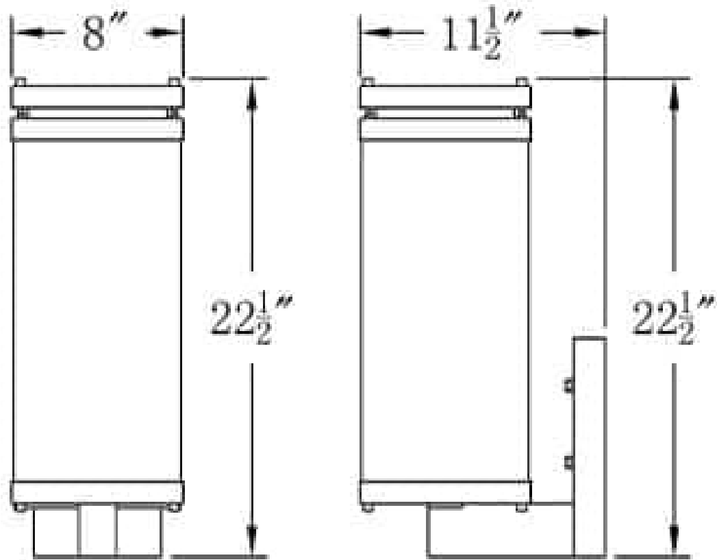
AU-24 (Front)
