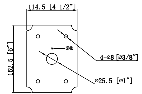
Same Aluminum Back plate As Gooseneck (T=4.0mm) (Front View)
