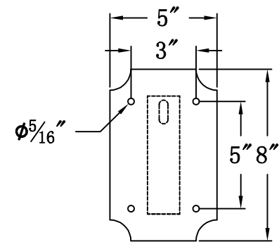
Mounting Plate
