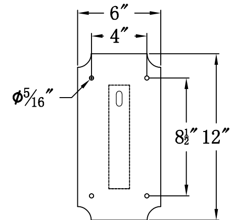
Mounting Plate
