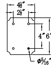
Front View of Mounting Plate
