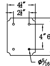
Front View of Mounting Plate
