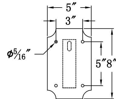
Mounting Plate
