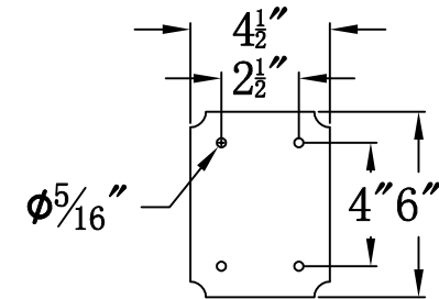
Front View of Mounting Plate
