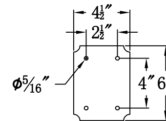
Front View of Mounting Plate
